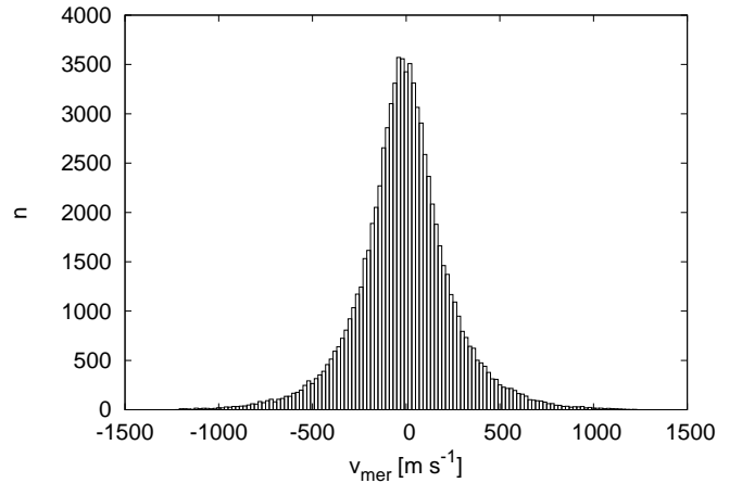
Fig. 5. Distribution of meridional velocities, v_{mer} , in bins 20 \text{ m s}^{-1} wide.
