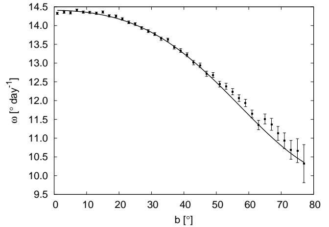
Fig. 2. Average solar rotation profile in 2^\circ bins of latitude, b , is shown with filled black squares and error-bars. The best fit solar rotation profile is shown with a solid black line.
