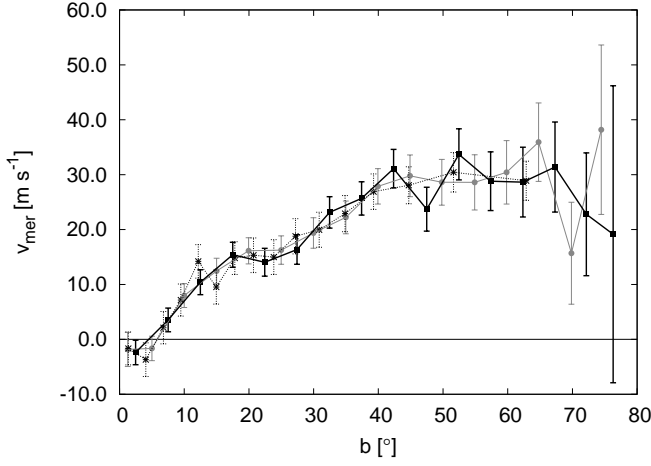
Fig. 6. Average meridional velocity, v_{mer} in 5^\circ bins of latitude, b , are shown with a thick black solid line and filled squares with error-bars. Values calculated with bins of the same width but with the first bin in the range 0^\circ – 2.5^\circ are shown with a grey solid line and filled circles with error-bars. v_{mer} averages in bins with constant number of data points ( n=5000 ) are shown with a dotted line and stars with error-bars.
