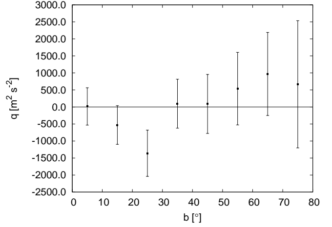
Fig. 7. Horizontal Reynolds stress in bins of 10^\circ in latitude, b , is shown with filled black squares with error-bars
