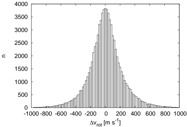
Fig. 3. Distribution of rotation velocity residuals, \Delta v_{rot} , in bins 20 \text{ m s}^{-1} wide.
