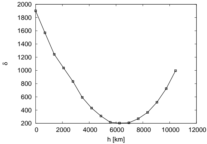
Fig. 1. \delta as a function of height, h , clearly shows a minimum value at around 6500 km above the photosphere.
