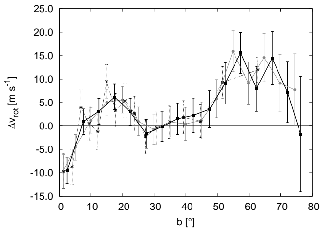
Fig. 4. Rotation velocity residuals, \Delta v_{rot} , in 5^\circ bins in latitude, b , are shown with a thick black solid line and filled squares with error-bars. Values calculated with bins of the same width but with the first bin in the range 0^\circ – 2.5^\circ are shown with a grey solid line and filled circles with error-bars. \Delta v_{rot} averages in bins with constant number of data points ( n=5000 ) are shown with a dotted line and stars with error-bars.
