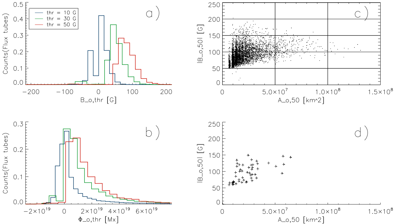
Figure 11. Distribution of the mean magnetic field densities (a) and magnetic flux (b), derived from all flux tubes extracted at 10 G (blue), 30 G (green), and 50 G (red). Positive values belong to the dominant polarity of their source coronal hole. Scatter plot of the mean magnetic field density of all flux tubes vs. their areas derived from all flux tubes extracted at 50 G (c), and derived for a single medium sized coronal hole (apparent on 2013/11/09; d).
